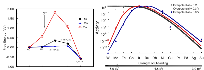
Figure 1. A) Free energies (at T=1000 K, P(H 2 )=1 atm, P(H 2 O) = 0.05 atm) for various elementary steps associated with electrochemical hydrogen oxidation, B) Normalized activity of various metal electro-catalysts. The activity is obtained with the parameters calculated in the first-principles calculations.
